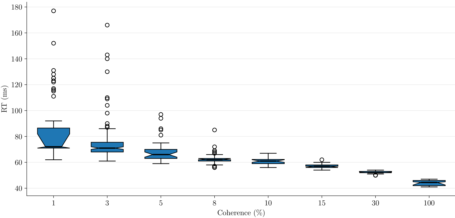
Correct RT Distributions for b = 0.20
